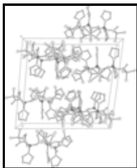
Fig. 2. Projection of packing diagram of 1 along the a -direction.
